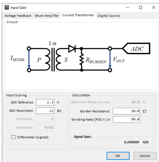
Figure 6: Shunt Amplifier Gain Calculator
