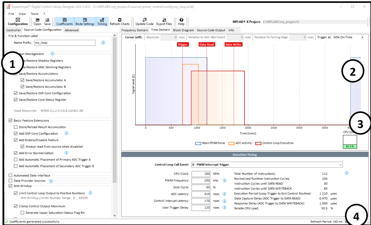
Figure 9: Code Generator Configuration and Timing Diagram
