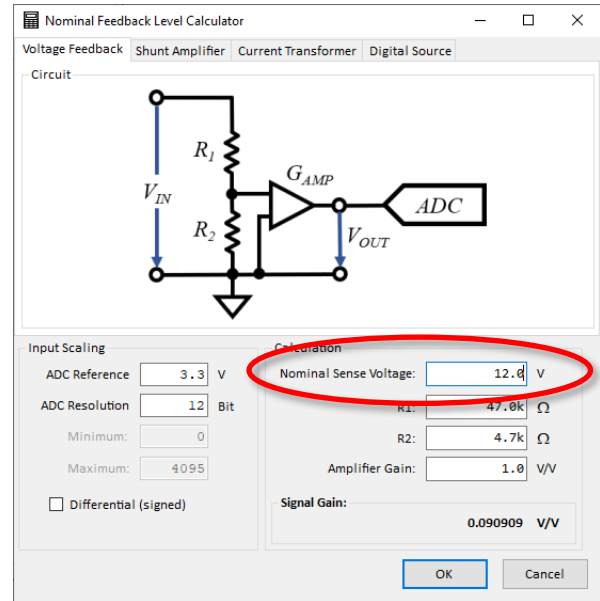
Figure 21: Nominal Feedback Level Calculator
