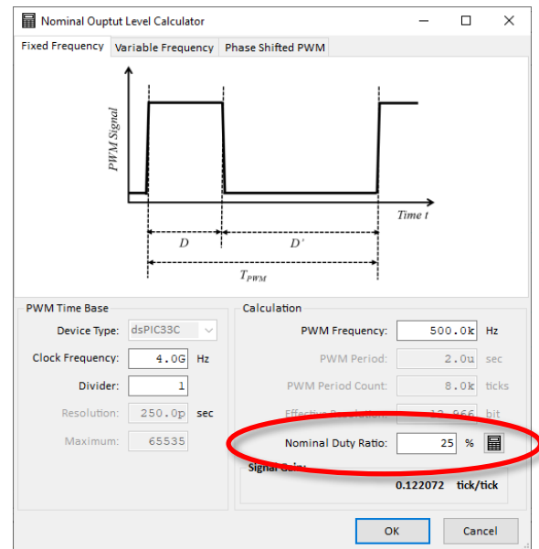
Figure 22: Nominal Control Output Level Calculator
