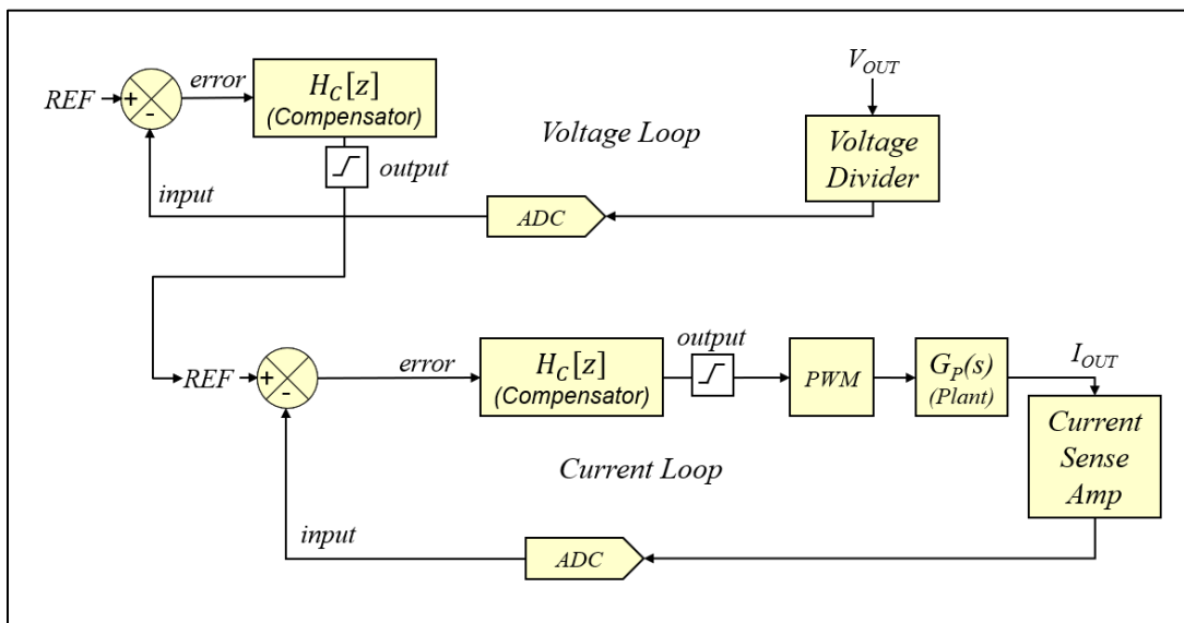
Figure 42: Standard Average Current Mode Control Feedback Loop Block Diagram
