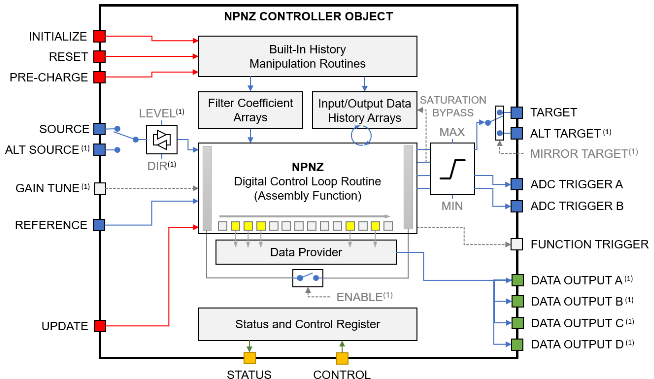
Figure 11: NPNZ16b_t Controller Object Block Diagram
