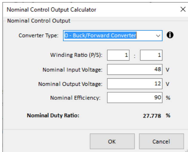
Figure 23: Duty Ratio Calculator
