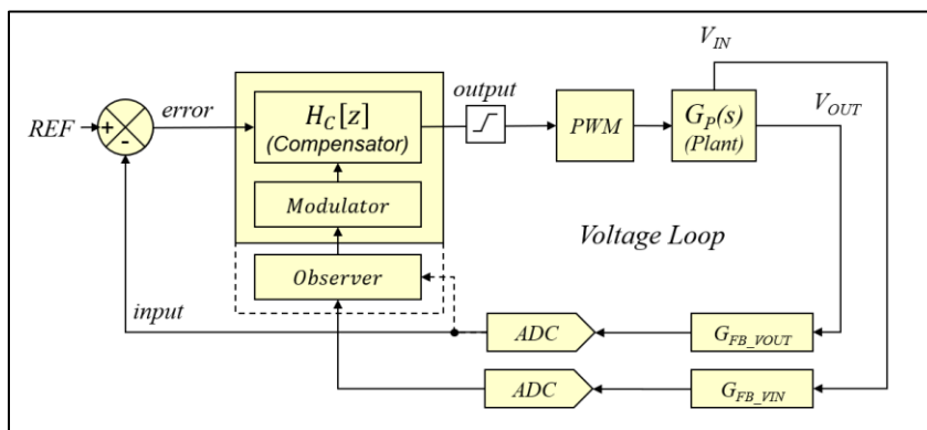
Figure 26: Adaptive Gain Control (Feed Forward) Block Diagram
