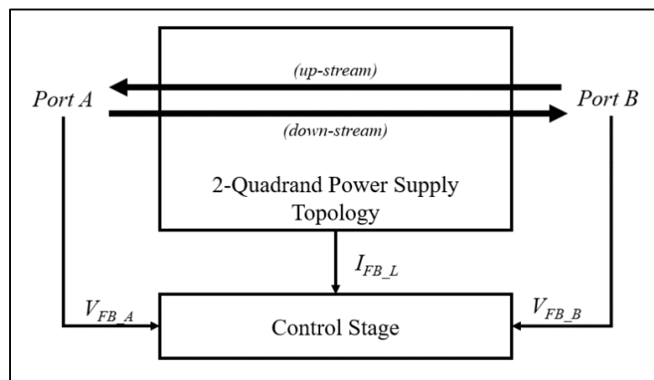
Figure 40: Bi-Directional Power Converter Block Diagram
