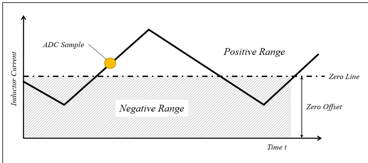
Figure 41: Bi-Directional Current Feedback Signal with Offset
