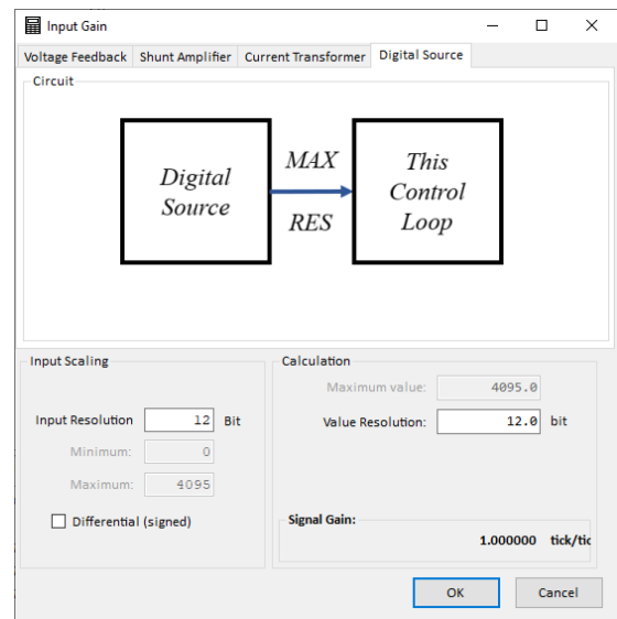
Figure 8: Digital Feedback Source Gain Calculator
