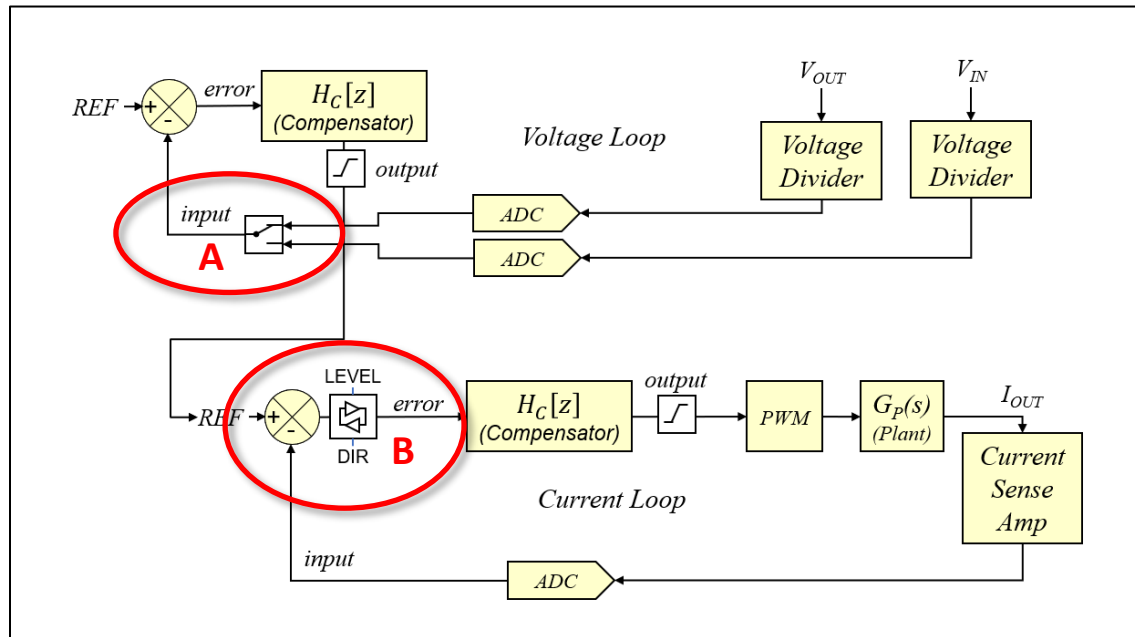
Figure 43: Bi-Directional Average Current Mode Control Feedback Loop Block Diagram
